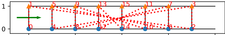
order='folded'
