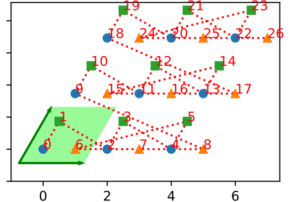
("grouped", [(0, 2), (1,)], [1, 0, 2])
