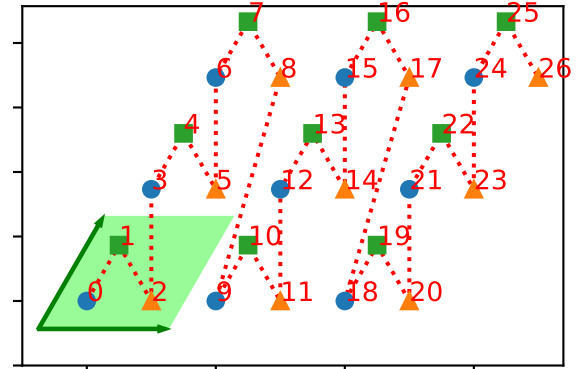
("grouped", [(0, 2, 1)], None)
