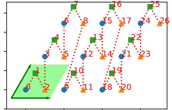
("grouped", [(0, 2, 1)], None)
