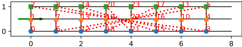
order='folded'
